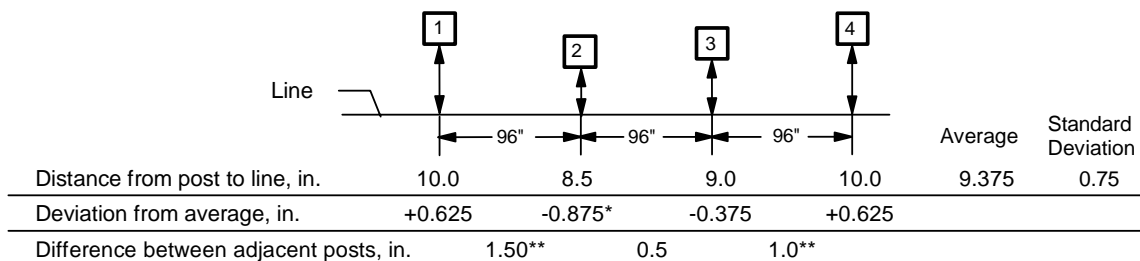
Figure 5 - Checking the alignment of posts 1, 2, 3 and 4 with a line that is equal distant (in this case 10.0 inches) from each corner post.
