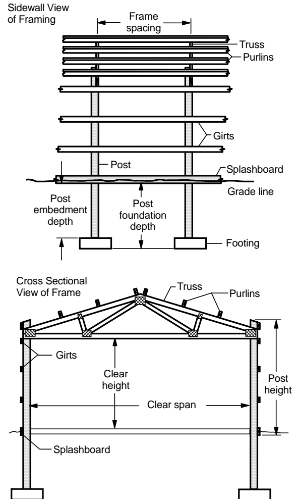
Figure 1 – Post-frame building terminology
