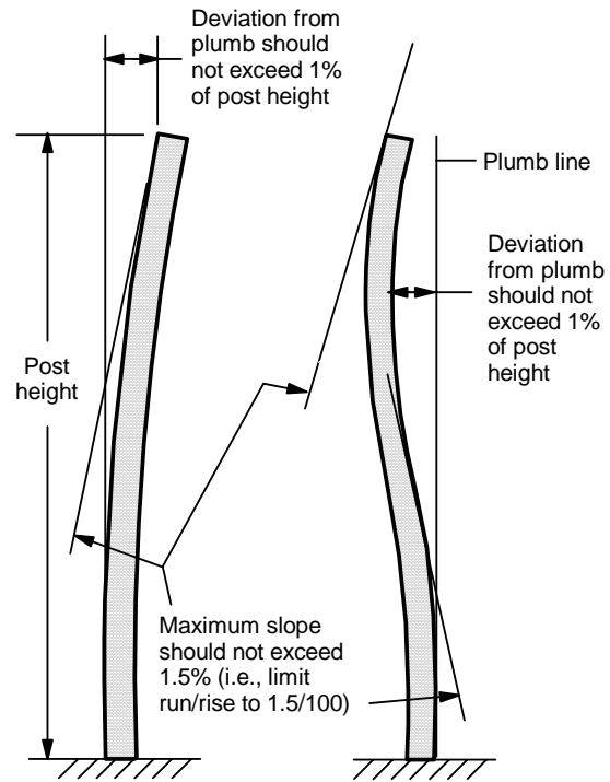
Figure 4 - Post plumbness criteria.
