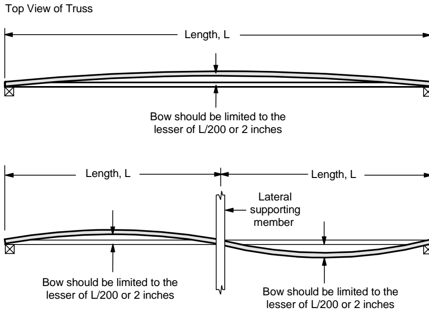
Figure 8 - Restrictions on overall truss bow and bow in truss members.
