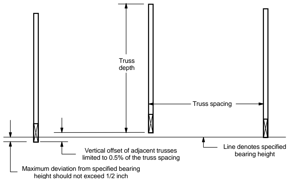
Figure 7 - Truss bearing height tolerances.
