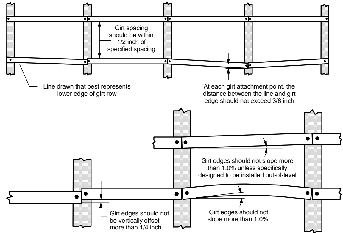
Figure 10 - Girt placement criteria.
