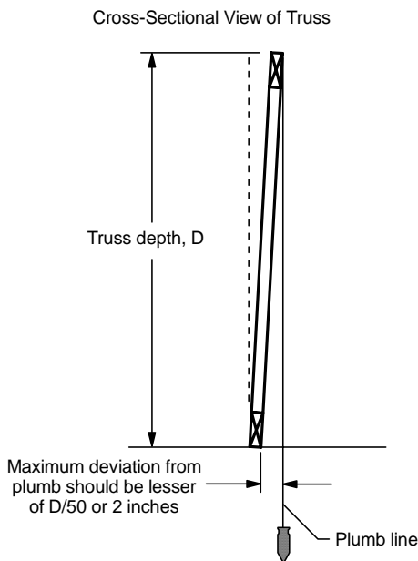
Figure 9 - Requirements for truss plumbness.
