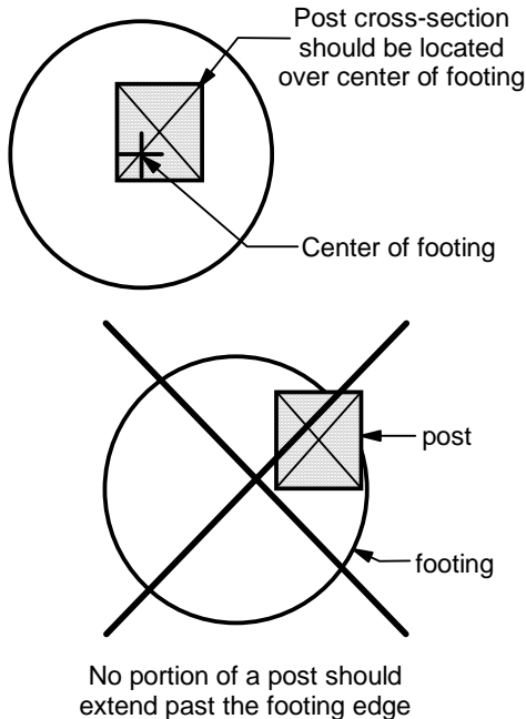
Figure 3 - Guidelines for post placement on footing.
