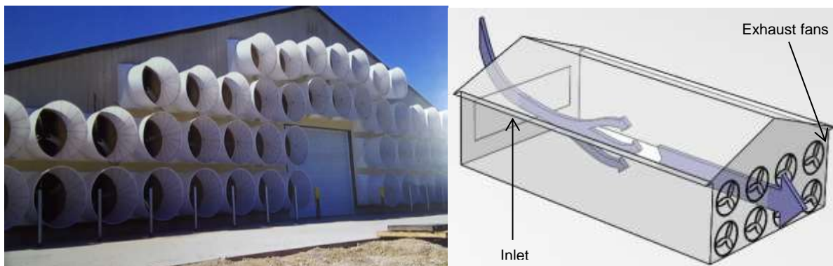
FIG. 5a. Tunnel-ventilated barns
